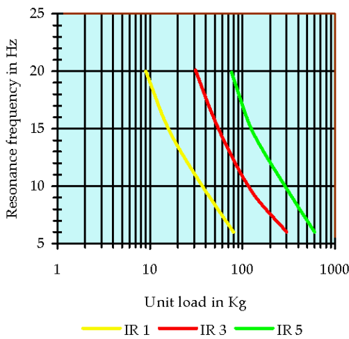
Load range under +/- 0,4mm
