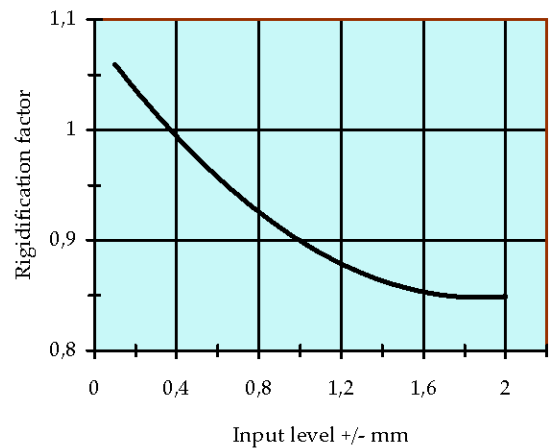
Typical dynamic rigidification behaviour
