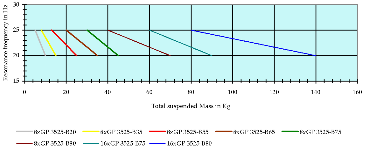
Load range for 8 or 16 isolators system under \pm 0,4\text{mm}
