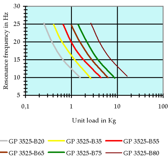
Radially load range under \pm 0,4\text{mm}
