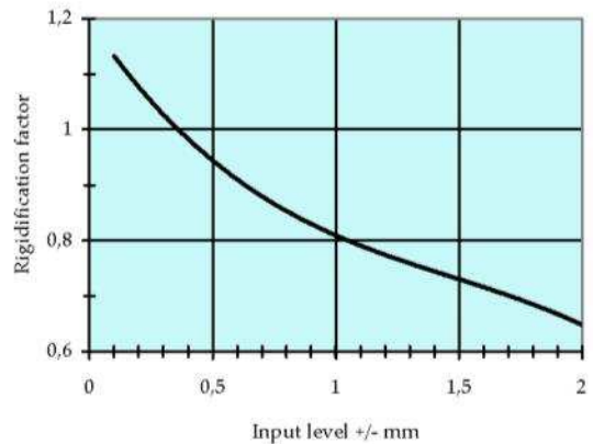
Typical dynamique rigidification behaviour
