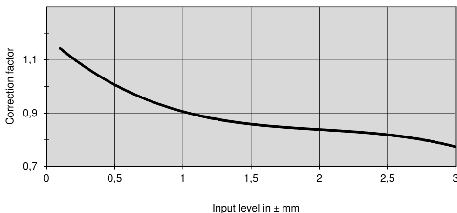
Typical dynamique rigidification behaviour
