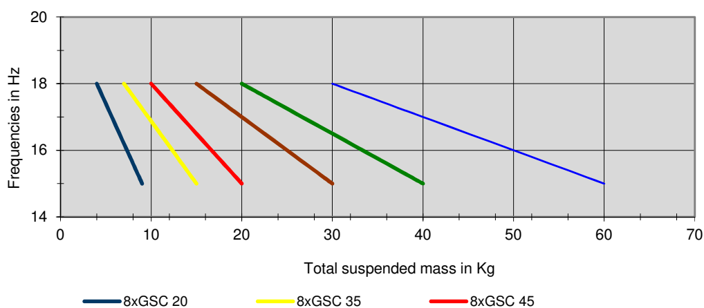
Load range with 8 dampers
